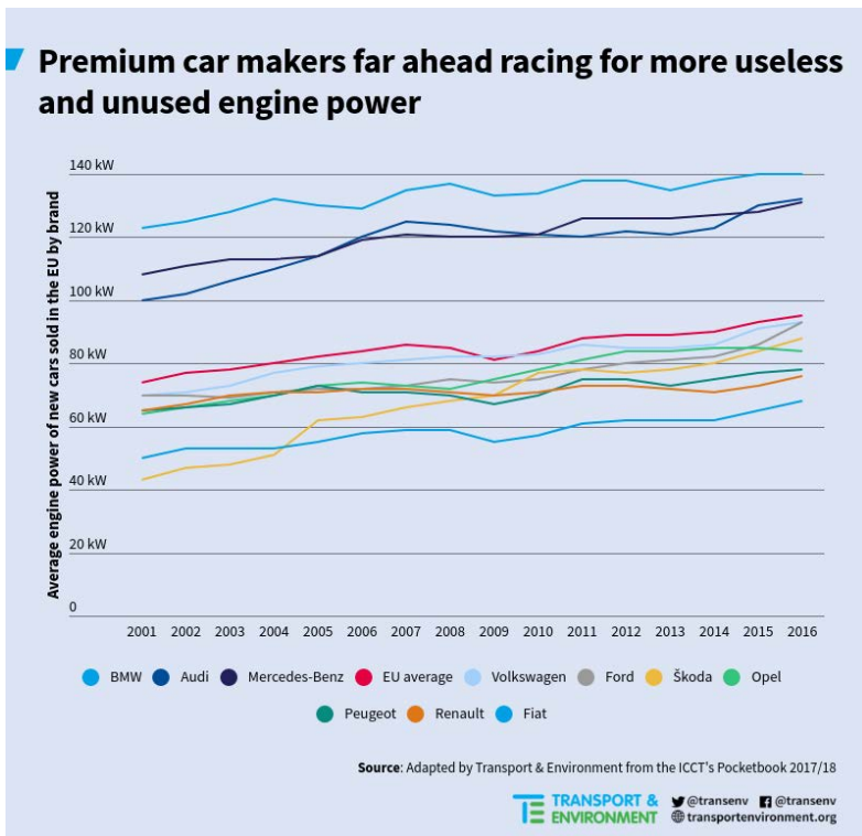
Figure 21 - Evolution of the average engine power for cars per brand in Europe from 2001 to 2016
