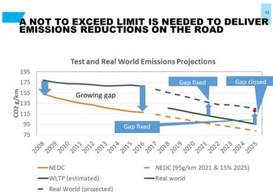
Figure 34 – Preventing manipulation of targets through real world measurements
