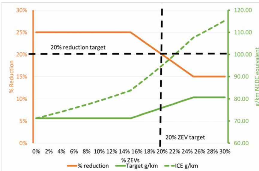
Figure 33 – Proposed two-way adjustment establishing a target for low and zero emissions vehicles
