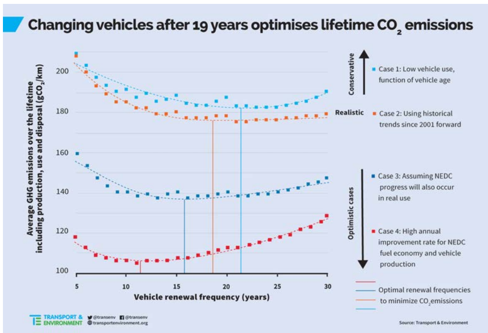
Figure 27 - Optimal renewal rate for a set of annual improvement rates
