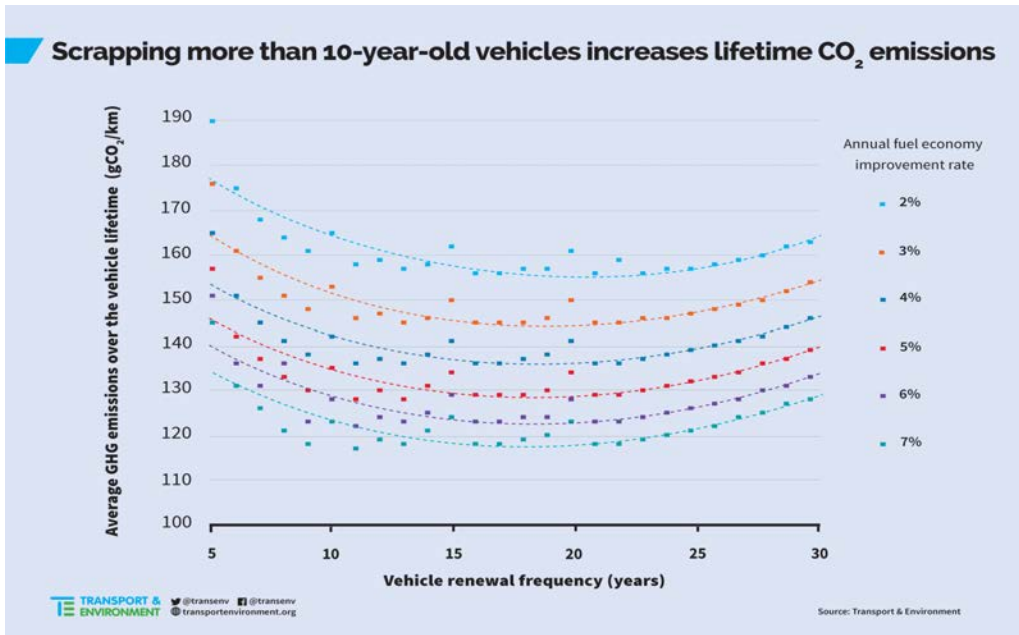
Figure 28 - Optimum vehicle renewal frequencies for different scenarios
